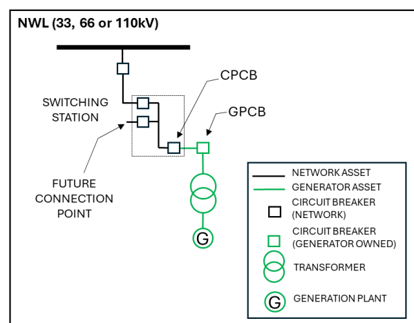
Figure 6: Subtransmission feeder (Owned by Network Waitaki)
