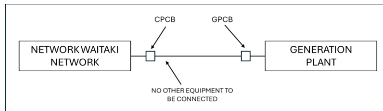
Figure 4: Connection Point Circuit Breaker
