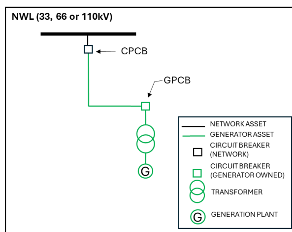
Figure 5: Dedicated subtransmission feeder (Owned by Generation Asset Owner)
