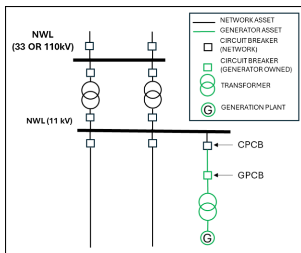
Figure 12: Distribution feeder (Owned by Generator Asset owner)
