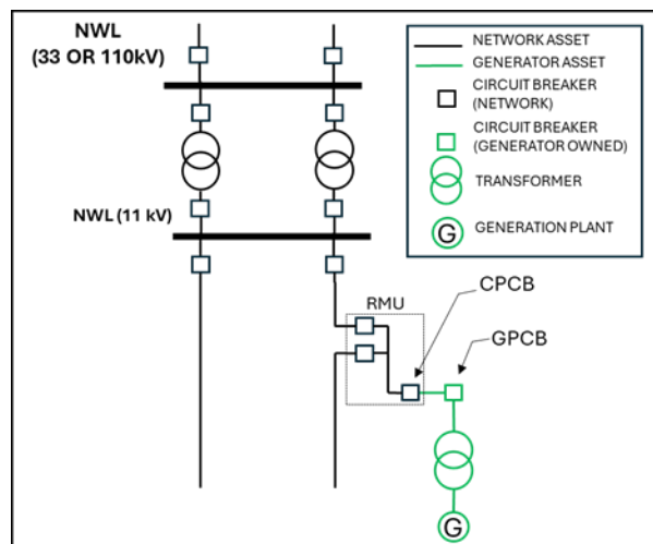
Figure 10: Distribution in-out from radial circuit
