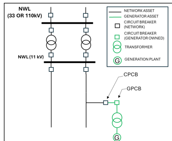
Figure 11: Distribution tee-off from radial circuit
