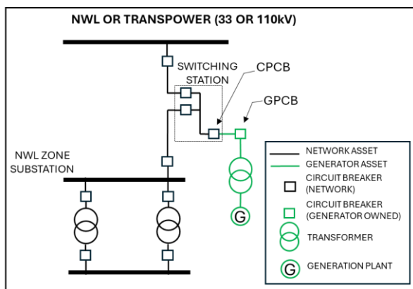
Figure 7: In-out from radial subtransmission feeder
