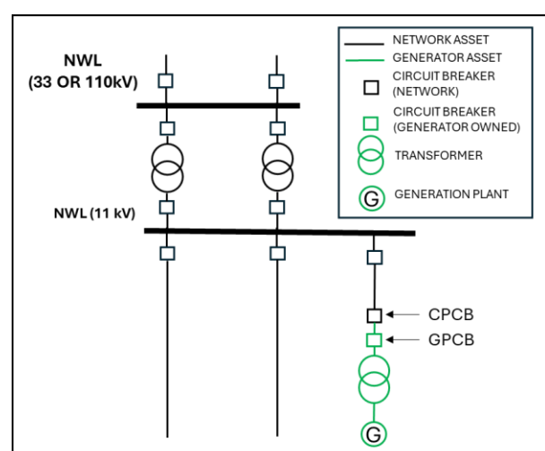
Figure 13: Distribution feeder
