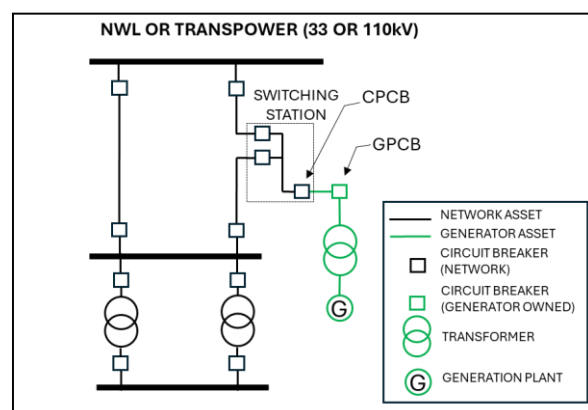
Figure 8: In-out from meshed subtransmission feeder
